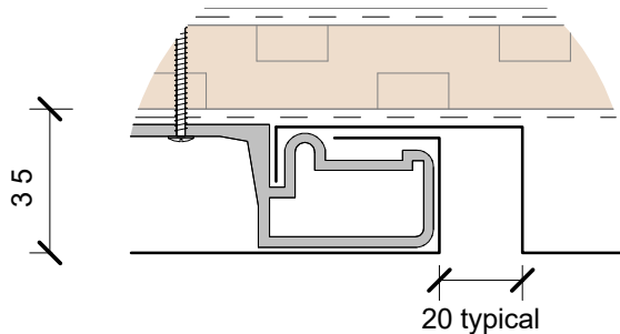
Euro Wall Flat Panel System vertical Scale 1:2
