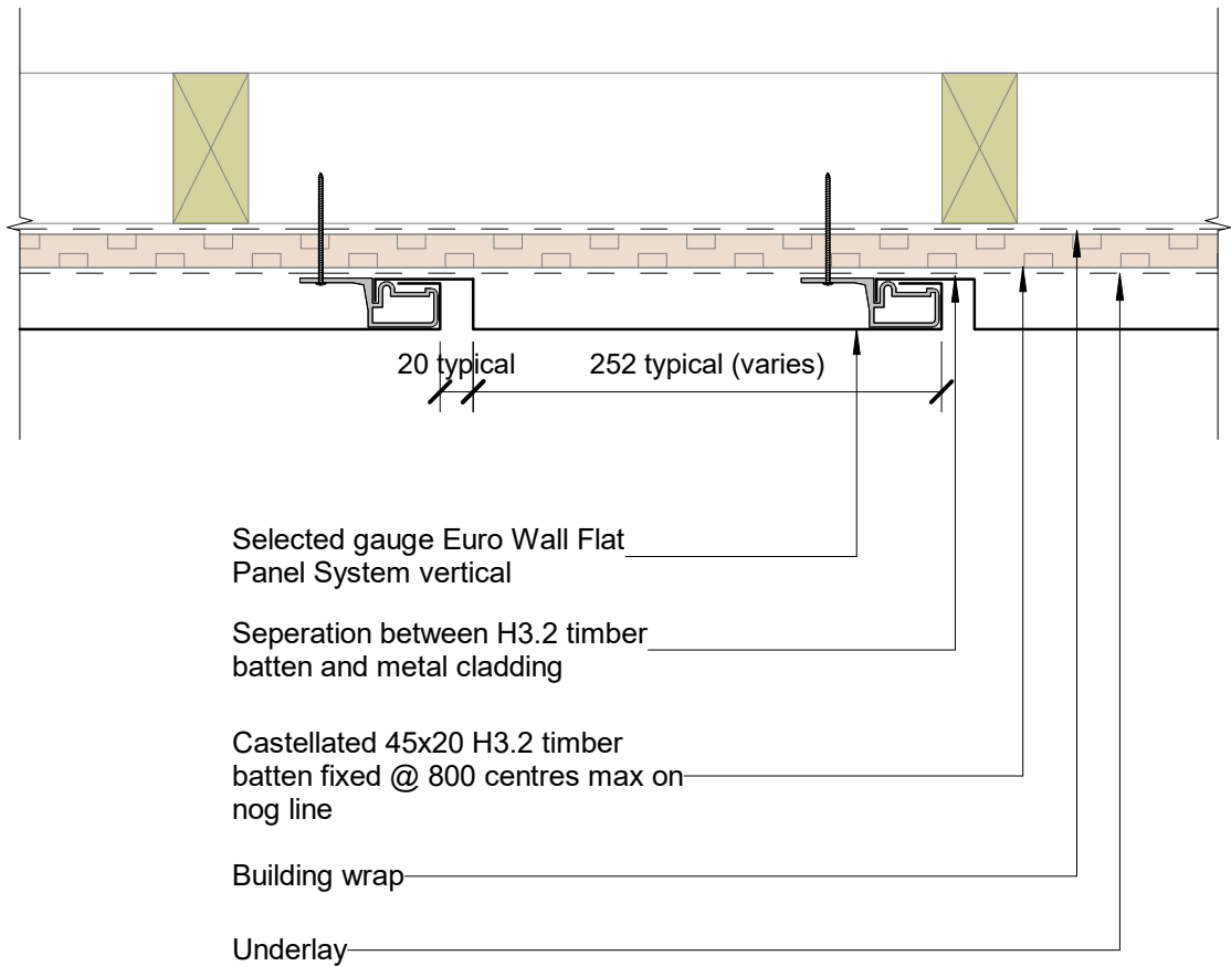
Scale 1:5
