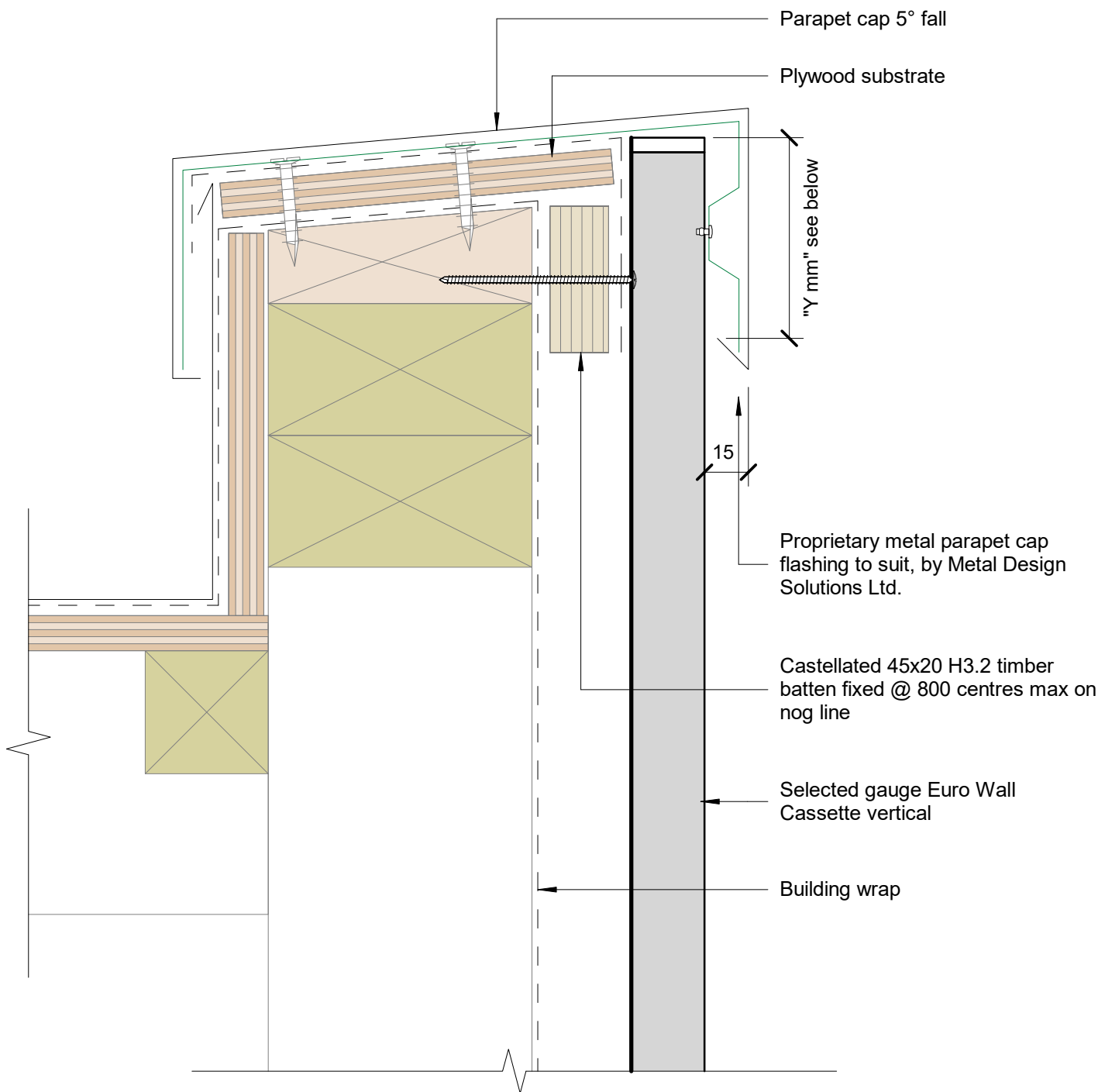
Parapet Typical (Y mm): excluding drip edge: 50mm in situation 1: Low, Medium and High wind zones 70mm in situation 2: Very High, Low, Medium and High wind zones 90mm in situation 3: Extra High wind zones
