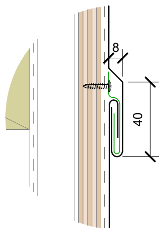
Euro Wall Lock Seam horizontal
